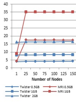
Figure 7. Twister vs. MPJ (Broadcasting 0.5~2GB data)
