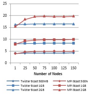
Figure 6. Twister vs. MPI (Broadcasting 0.5~2GB data)
