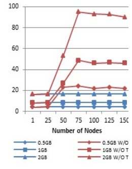
Figure 9. Twister Chain with/without topology-awareness
