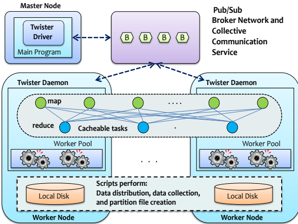
Figure 4. Initial Twister architecture
