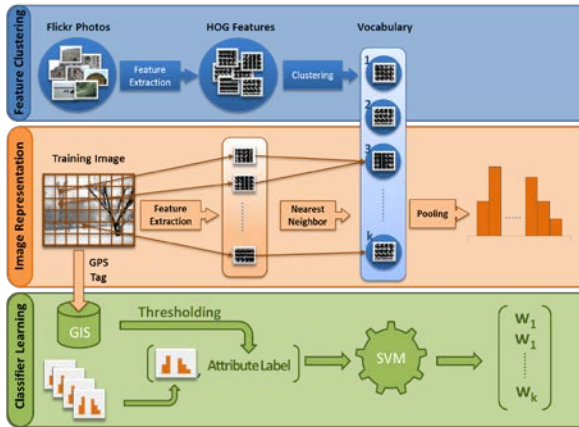
Figure 1. Workflow of the vocabulary learning application.
