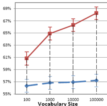
Figure 10. Accuracy of urbanicity (red solid) and elevation gradient (blue dashed) classifiers for
