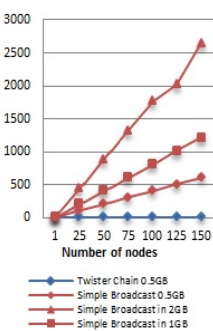
Figure 5. Twister Chain vs. Simple Broadcasting
