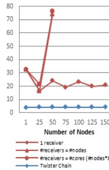
Figure 8. Twister vs. Spark (Broadcasting 0.5GB data)
