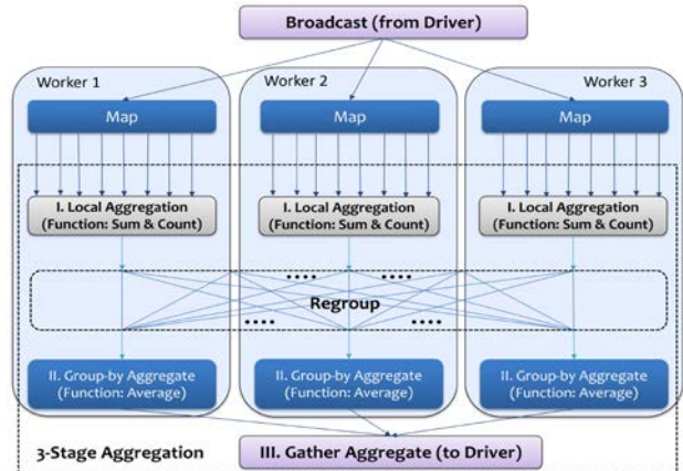
Figure 2. Image clustering control flow in Twister with the new local aggregation feature in Map stage.
