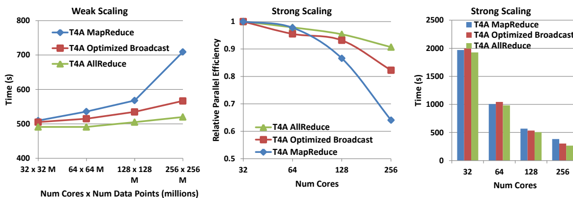
Figure 16 Twister4Azure K-means Clustering comparison with Map-AllReduce. 500 Centroids (clusters). 20 Dimensions. 10 iterations. Left: Weak scaling 32 to 256 Million data points. Right: 128 Million data points. Parallel efficiency relative to the 32
