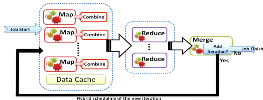
Figure 3 Twitter4Azure MapReduce-MergeBroadcast compute/data flow
