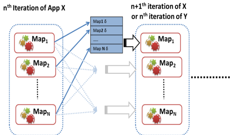
Figure 6 Map-AllGather Collective
