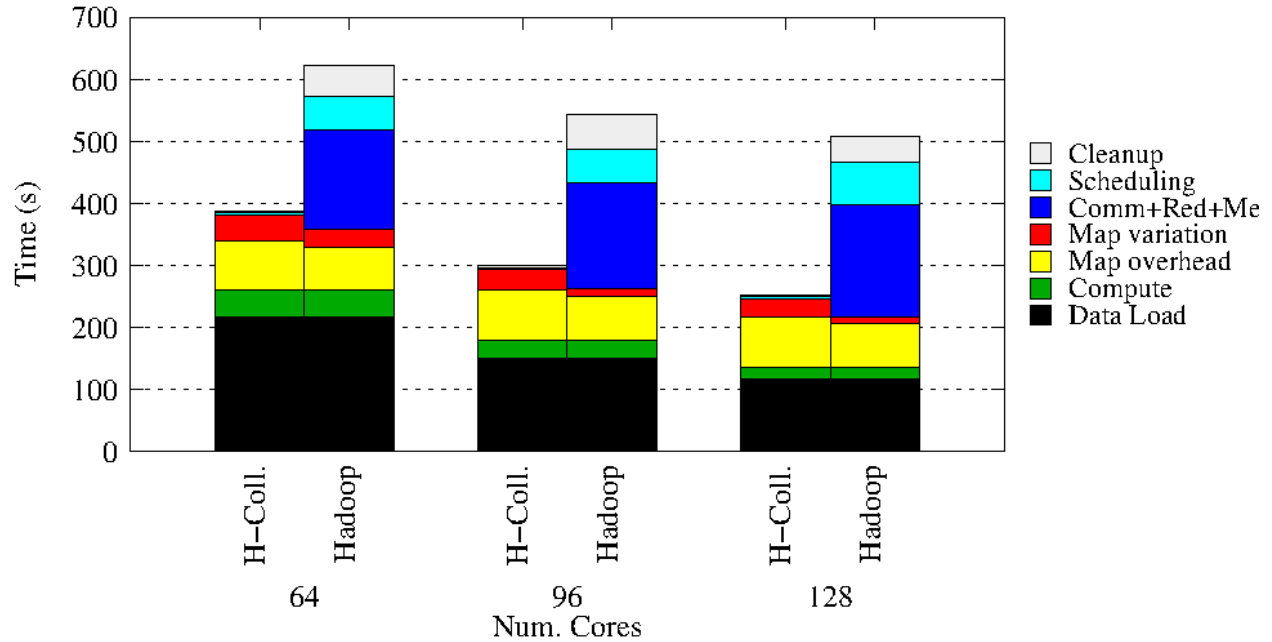
Figure 12 MDS Hadoop using only the BC Calculation MapReduce job per iteration to highlight the overheads. 20 iterations, 51200 data points
