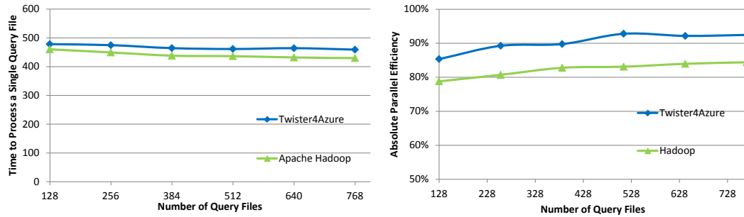
Figure 13. Twister4Azure BLAST performance. Left (a) : Time to process a single query file. Right (b): Absolute parallel efficiency
