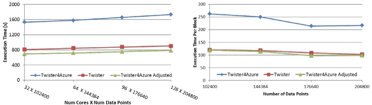
Figure 8. Left (a): MDS weak scaling where we the workload per core is constant. Ideal is a straight horizontal line. Right (b): Data size scaling using 128 Azure small instances/cores, 20 iterations
