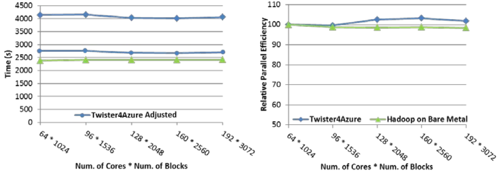
Figure 12. Twister4Azure SWG performance. Left : Raw and adjusted execution times. Right: Parallel efficiency relative to the 64*1024 test case
