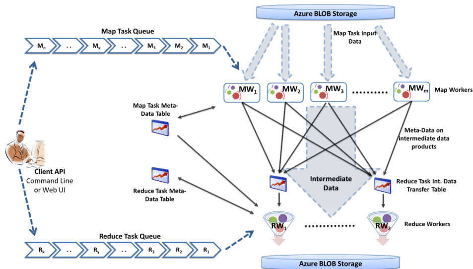
Figure 1. MRRoles4Azure Architecture [4]
