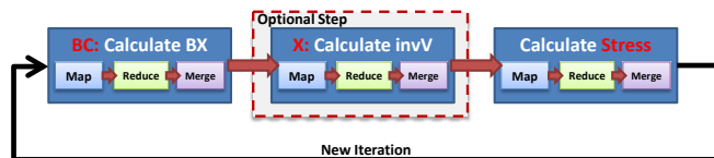
Figure 7. Twister4Azure Multi-Dimensional Scaling
