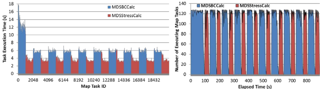
Figure 9. Twister4Azure Map Task histograms for MDS of 204800 data points on 32 Azure Large Instances (graphed only 10 iterations out of 20). Left (a): Map task execution time histogram. Two adjoining bars (blue and red) represent an iteration (2048 tasks per iteration), where each bar represent the different applications inside the iteration. Right (b): Number of executing Map Tasks in the cluster at a given moment. Two adjoining bars (blue and red) represent an iteration.
