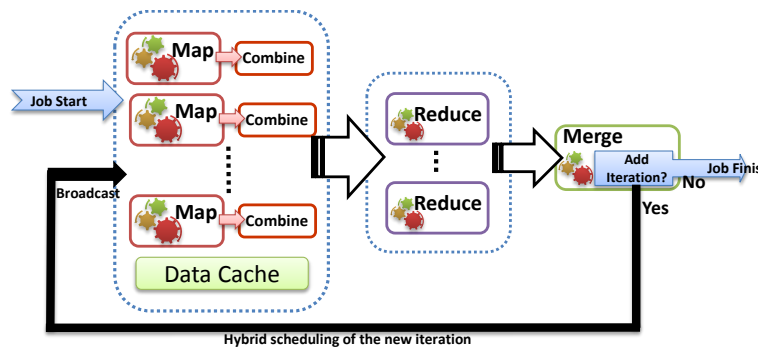
Figure 4. Twister4Azure iterative MapReduce programming model
