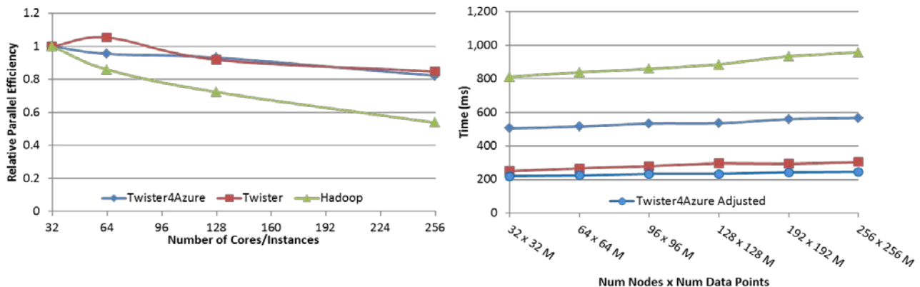
Figure 10. KMeansClustering Scalability. Left(a): Relative parallel efficiency of strong scaling using 128 million data points. Right(b): Weak scaling. Workload per core is kept constant (ideal is a straight horizontal line).
