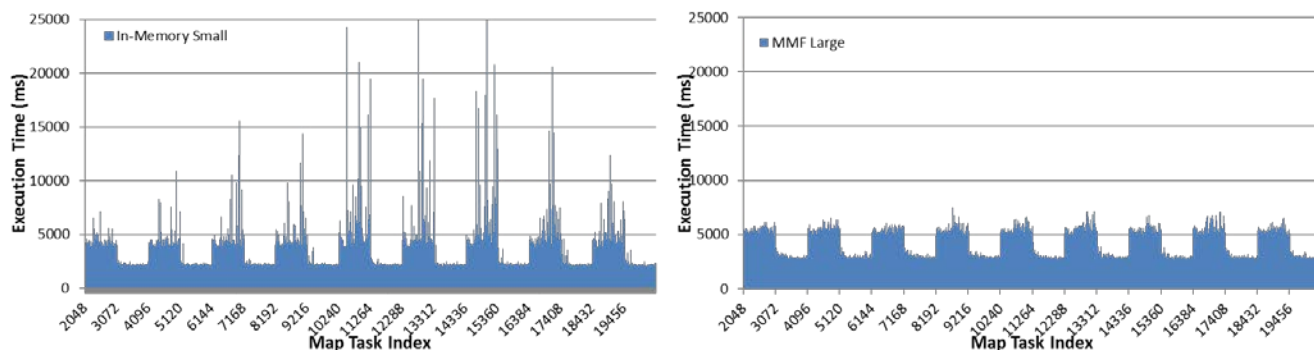
Figure 14. Execution traces of MDS iterative MapReduce computations using Twister4Azure showing the execution time of tasks in each iteration. The taller bars represent the MDSBCCalc computation, while the shorter bars represent the MDSStressCalc computation. A pair of BCCalc and StressCalc bars represents an iteration. Left (a): Using in-memory caching on small instances. Right (b): Using Memory-Mapped file based caching on Large instances.
