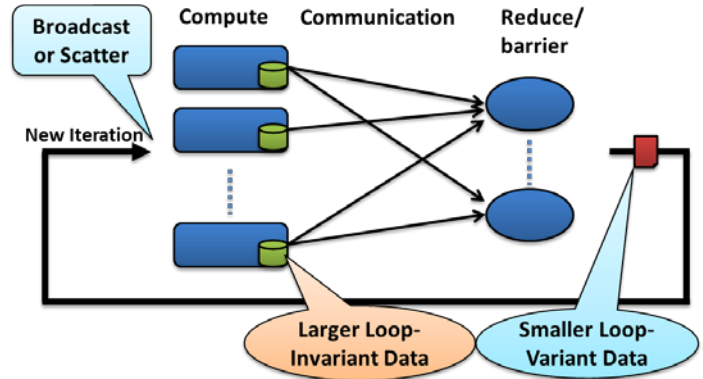
Figure 3. Structure of a typical data-intensive iterative application
