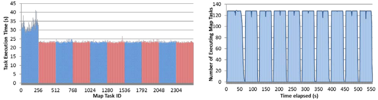
Figure 11. Twister4Azure Map Task histograms for KMeans Clustering 128 million data points on 128 Azure small instances. Left(a): Map task execution time histogram Right(c): Number of executing Map Tasks in the cluster at a given moment
