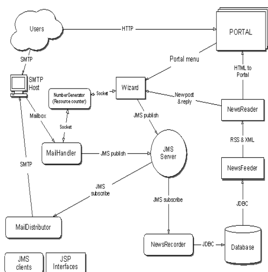
Figure 1: OKC's newsgroup architecture supports both email and JSP clients and readers.
