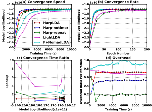
Figure 7: Performance on bigram with 10 \times 8 K=500
