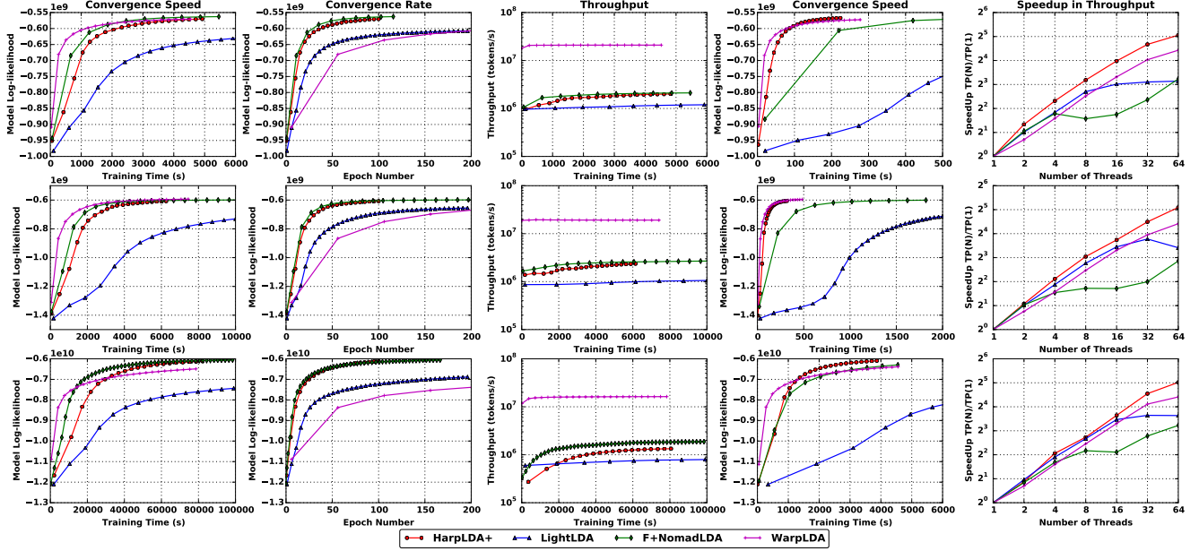
Figure 4: Single Node Performance with 3 rows corresponding to 3 datasets nytimes ( K = 1000 ), pubmed2m ( K = 1000 ), enwiki ( K = 10000 ) respectively. The columns are different observables with columns 1 to 3 reporting sequential single thread measurements and column 4 with 32 threads. Column 5 plots the results against different thread counts. Each column corresponds to an evaluation metric denoted in the title.
