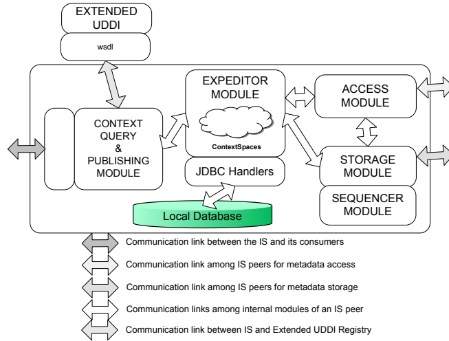
Fig.2. Architecture of an Information Service running on each peer
