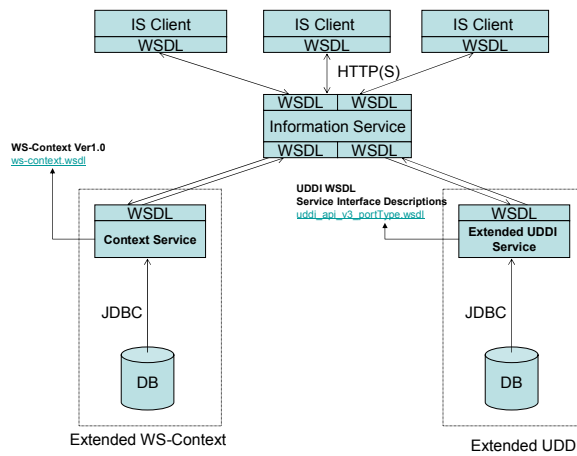
Fig.1. Our design integrates both UDDI and WS-Context Metadata Services to provide uniform programming interface to service metadata.
