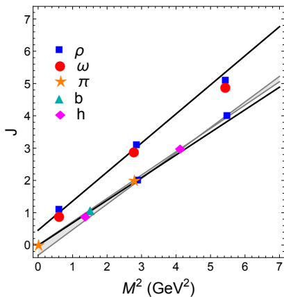
FIG. 14. Chew-Frautchi plot including the \pi , b , h and \rho excitations and quark model states 2^{--} and 4^{--} . The black lines show the trajectories \alpha(t) = 0.7(t - m_\pi^2) and \alpha(t) = 1 + 0.9(t - m_\rho^2) .
