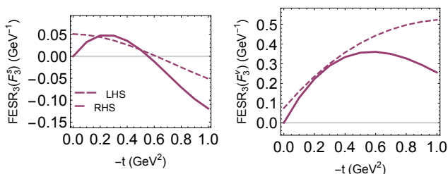
FIG. 8. LHS and RHS of the FESR for the two isospin components of the definite parity, singularity free t -channel nucleon-helicity flip amplitude F_3 (see Eq. (43)).
