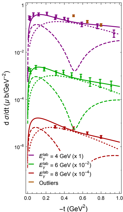
FIG. 12. High energy \gamma p \rightarrow \eta p data compared to the fitted Regge model. The dotted (dashed) line shows the isovector (isoscalar) contribution. The solid line represents the full Regge model. Data are from Refs [14, 15]. The three data points in brown from Dewire et al. [15] at E_\gamma^{\text{lab}} = 4 GeV were excluded from the fit due to a systematic inconsistency.
