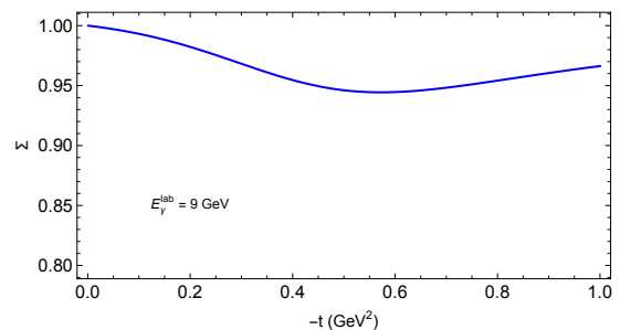
FIG. 13. Predictions for the beam asymmetry at E_\gamma^{\text{lab}} = 9 GeV for the conservative model.
