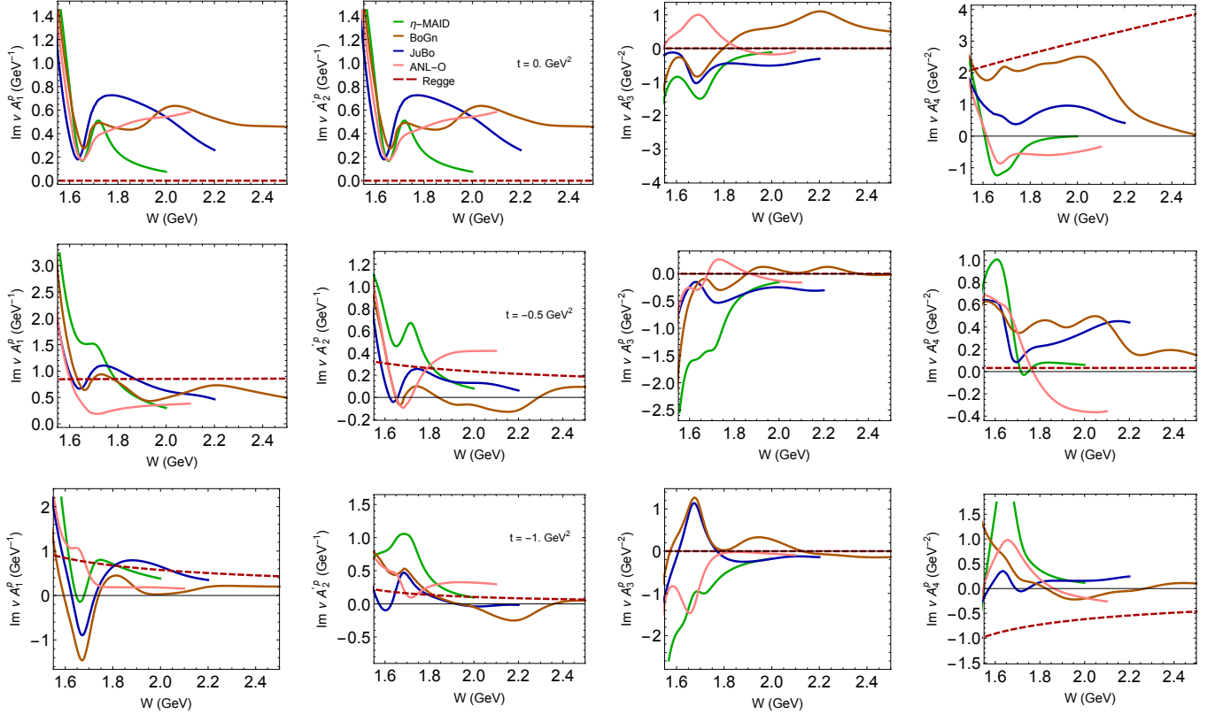
FIG. 10. Comparison of the proton-target amplitudes A_i^p = A_i^s + A_i^v of the high-energy Regge prediction to a number of resonance-region models for t = 0, -0.5 and -1 GeV 2 from top to bottom. The models have been constructed using their l \leq 5 multipoles only.
