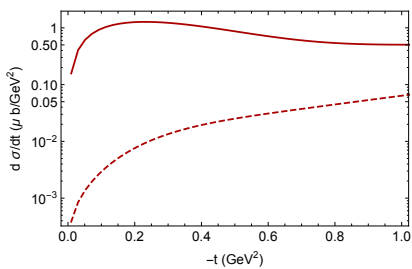
FIG. 11. The \eta -MAID differential cross section at W = 2.0 GeV. The solid line is the full model, and the dashed line shows the A_3 contribution.
