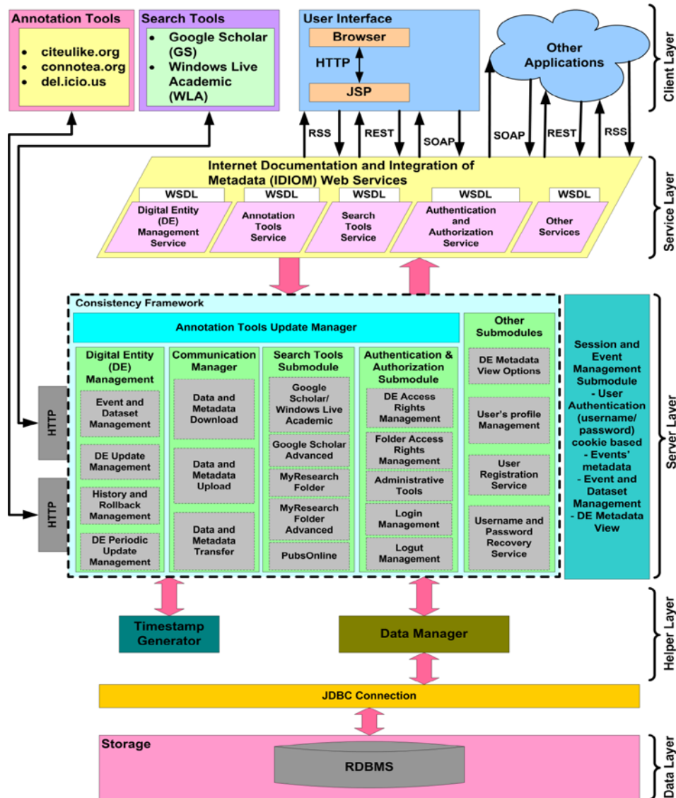
Fig. 7. Internet Documentation and Integration of Metadata (IDIOM) Architecture
