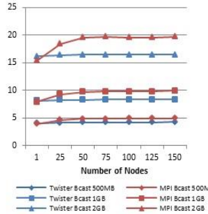
Figure 6. Twister vs. MPI (Broadcasting 0.5~2GB data)
