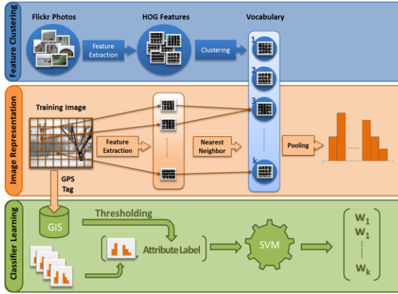
Figure 1. Workflow of the vocabulary learning application.
