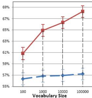
Figure 10. Accuracy of urbanicity (red solid) and elevation gradient (blue dashed) classifiers for increasing vocabulary sizes.
