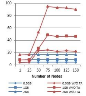
Figure 9. Twister Chain with/without topology-awareness
