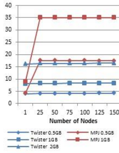
Figure 7. Twister vs. MPJ (Broadcasting 0.5~2GB data)
