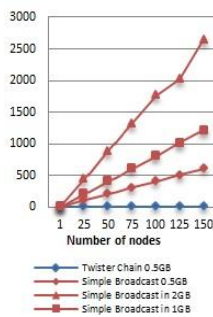
Figure 5. Twister Chain vs. Simple Broadcasting
