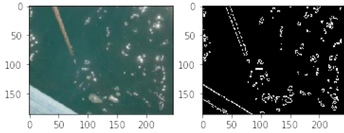
Figure 16: Edge Detection 4
