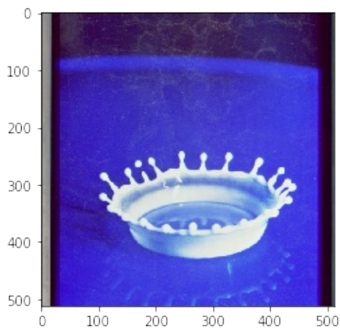
Figure 1: Image display
