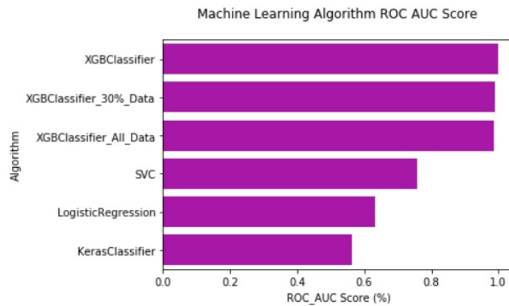
Figure 31: scikit-learn
