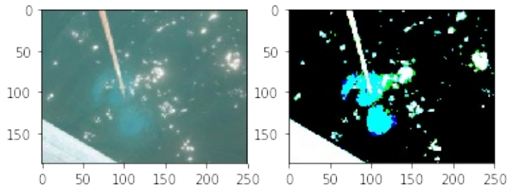
Figure 11: Threshold 3
