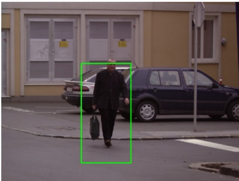
Figure 55: Example
