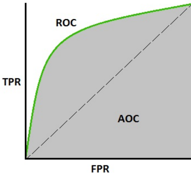
Figure 30: scikit-learn
