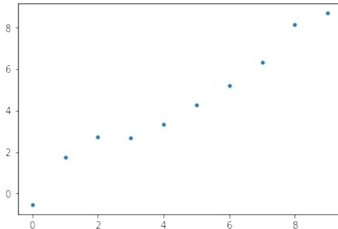
Figure 21: Result 1
