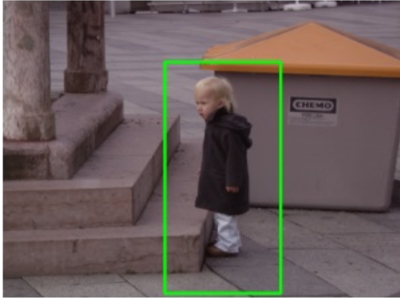
Figure 38: Pedestrian Detected
