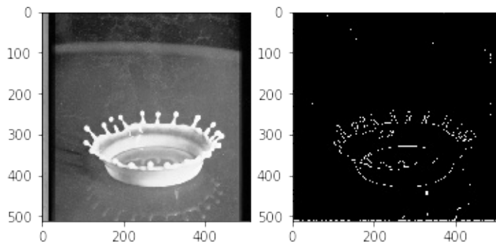
Figure 6: Edge detection
