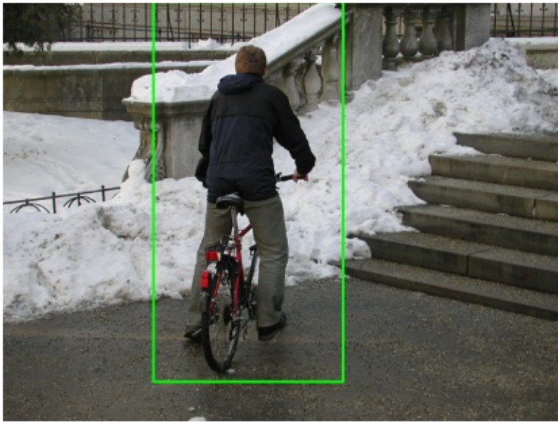
Figure 59: Example
