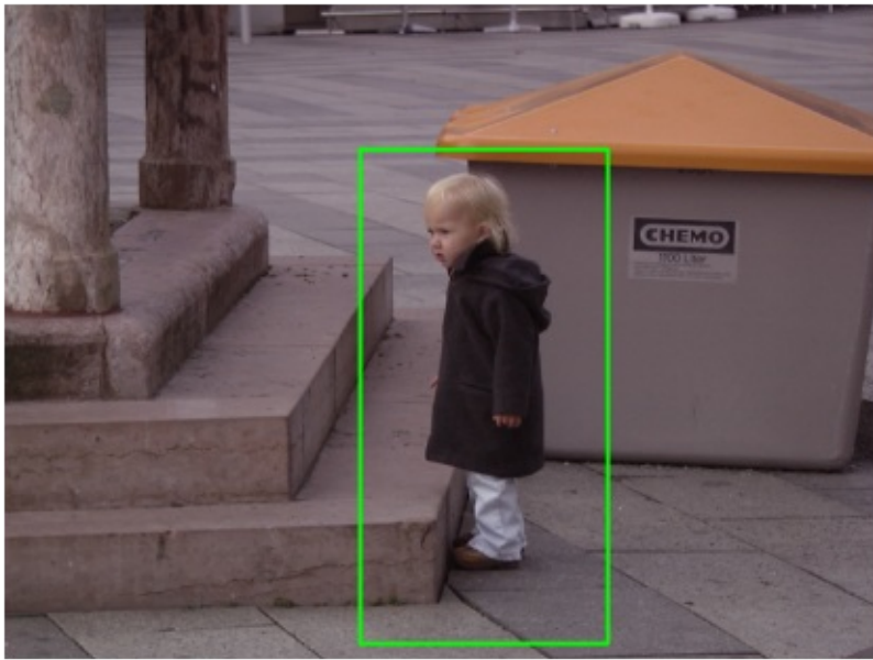
Figure 57: Example
