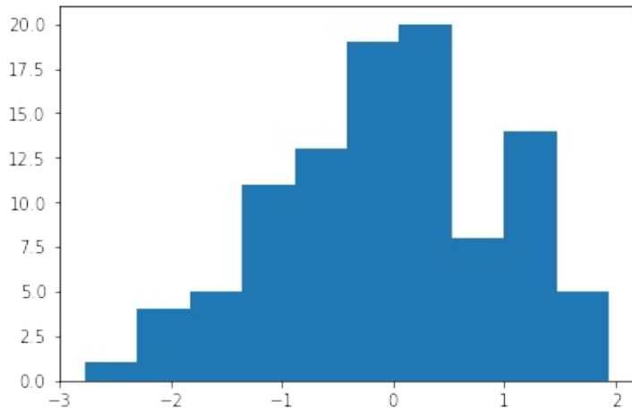
Figure 18: Histogram 1
