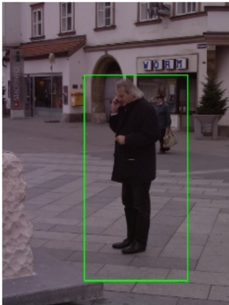
Figure 63: Example
