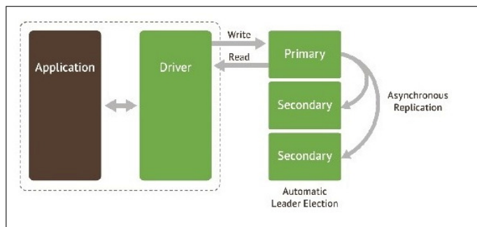
Fig. 2. MongoDB replica sets [2].
