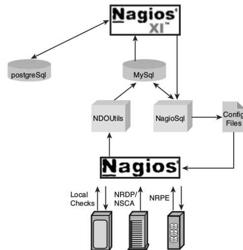
Fig. 1. Nagios Architecture [4].
