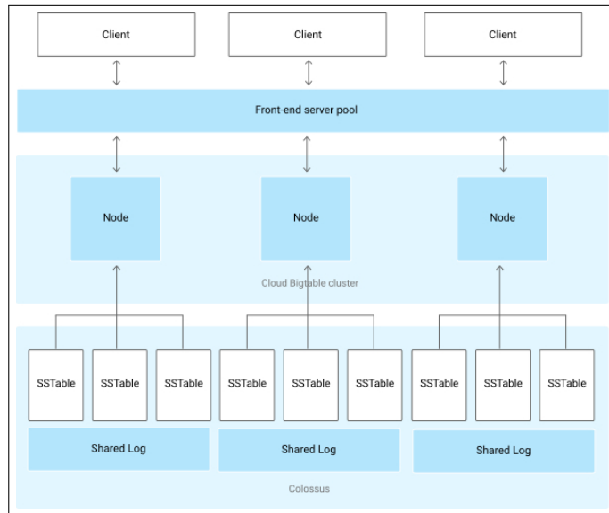
Fig. 2. Bigtable Architecture [5]
