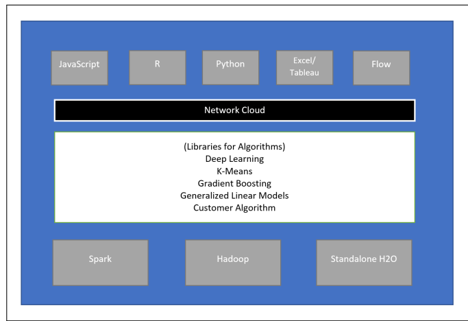
Fig. 1. H2O Architecture[4]
