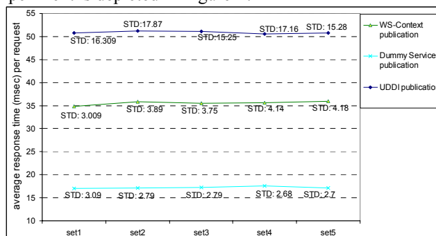
Figure 2. Average Response Time Graph for Publication Requests.
